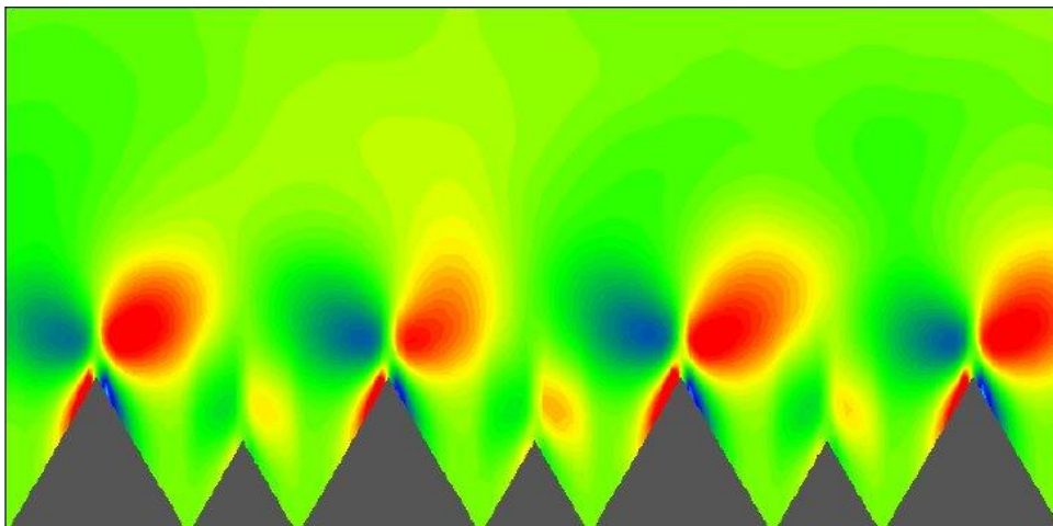
Figure 1: Mean streamwise vorticities for 60° riblets of brother/sister configuration
